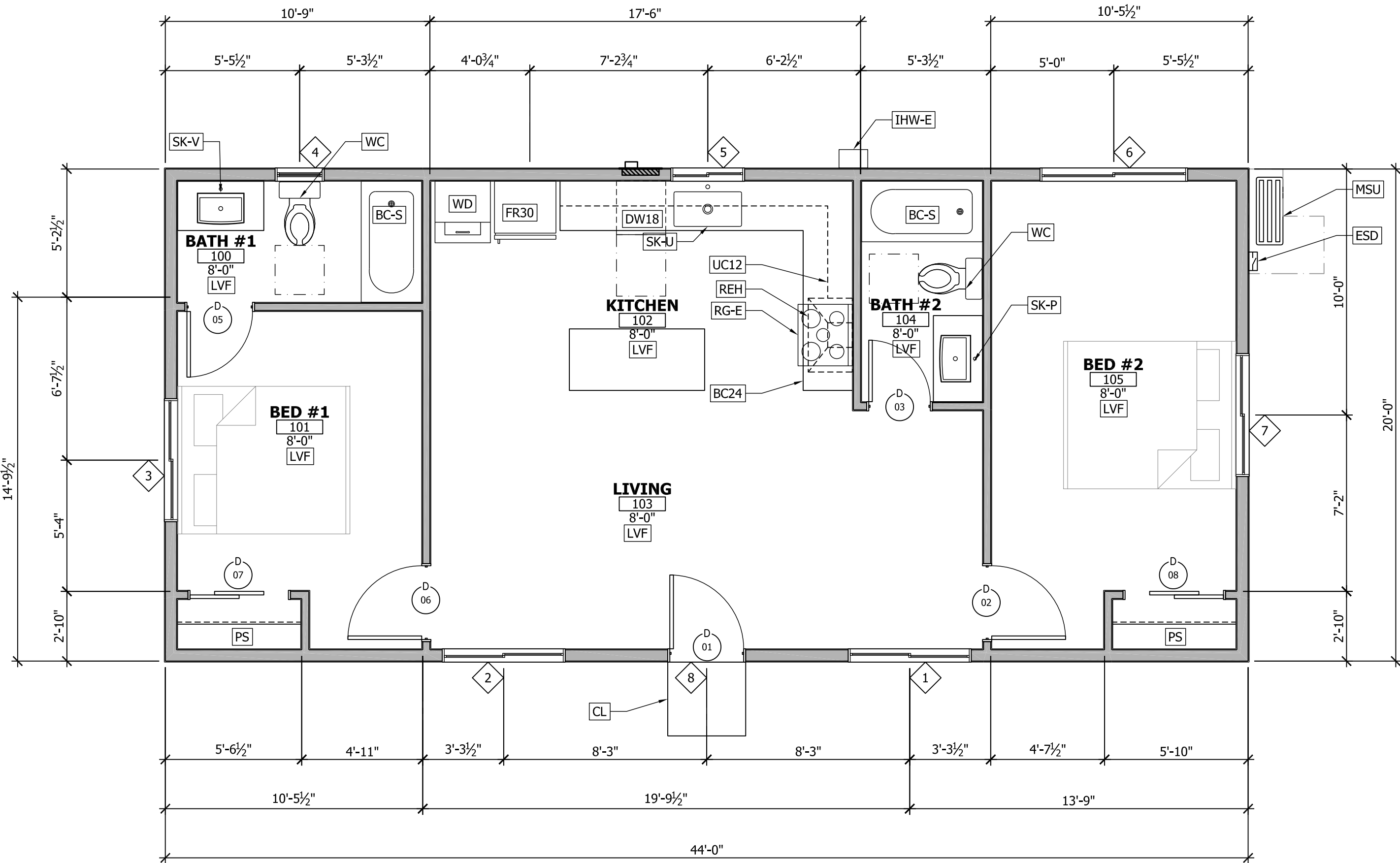
1 FLOOR PLAN 1 1/4" = 1'-0"
